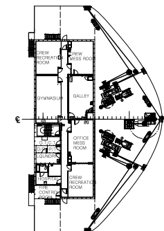
UPPER DECK
