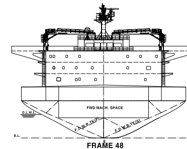
FRAME 48
