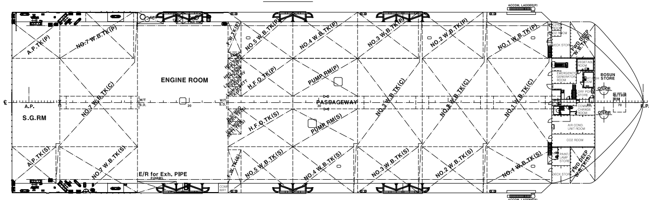
BELOW PASSAGE LEVEL (5.16 m A/B)
